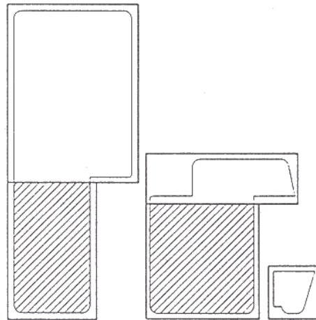
Cross-sectional view of side/top frame with casement
