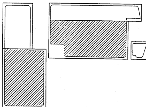
Cross-sectional view of side/top frame and casement
