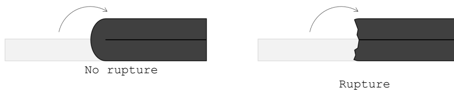
Figure 7 – brittle test (bending test)
