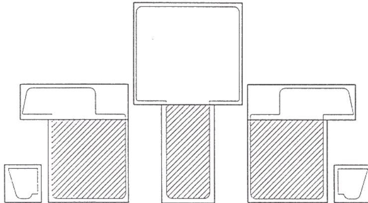
Cross-sectional view of mullion with casements
