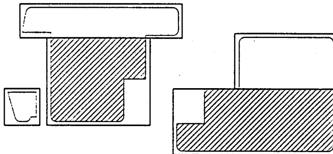
Cross-sectional view of side/top frame with casement
