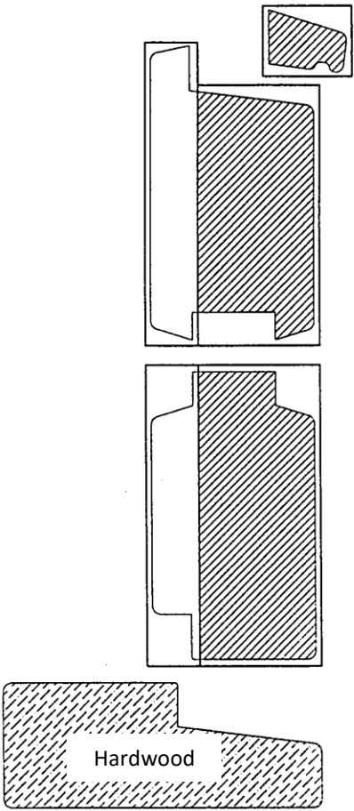
Cross-sectional view of sill and casement
