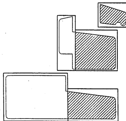
Cross-sectional view of sill and casement
