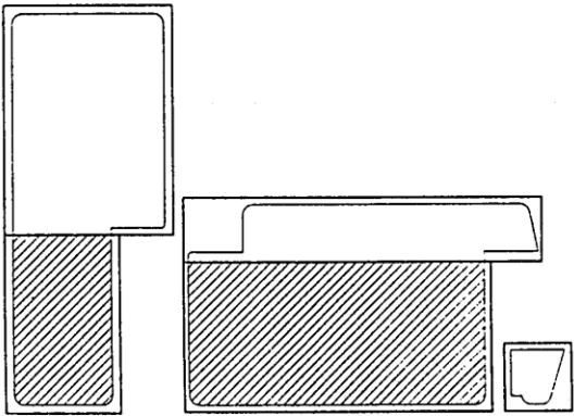
Cross-sectional view of side/top frame and casement
